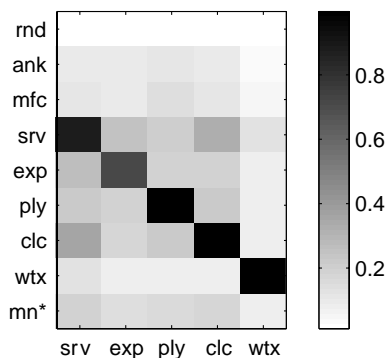
Figure 1: Top-N ranking agreement scores from table 3 plotted as a grayscale image.
